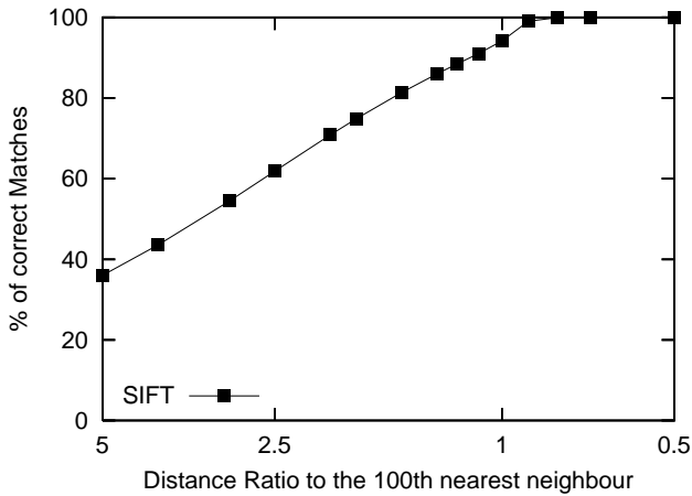
Fig. 3. The cumulative distribution of correct matches based on contrast.
