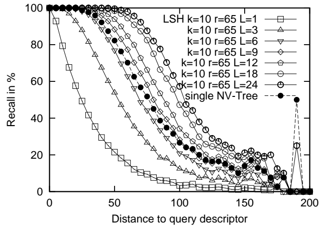
Fig. 13. Recall for LSH ( k=10, r=65 ) with varying number of tables.
