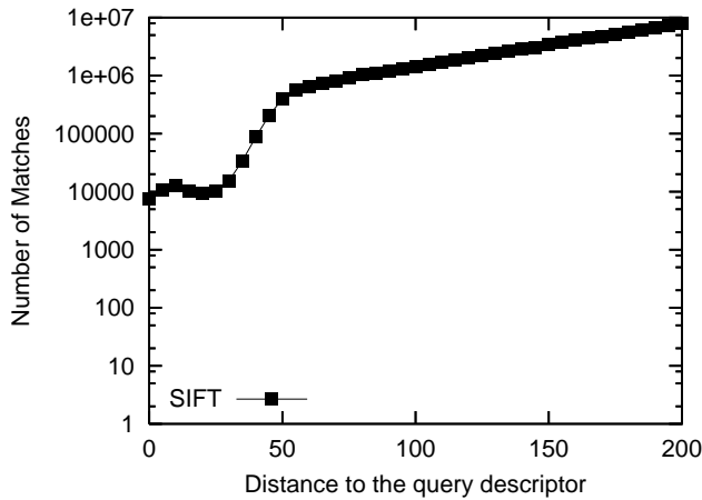
Fig. 1. The distribution of all neighbors based on distance to the query descriptor.
