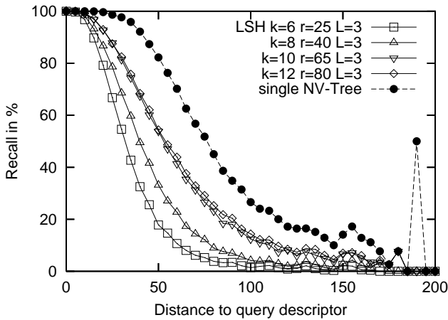
Fig. 12. Recall for different LSH setups (varying word size and radius) with 3 Hashtables.
