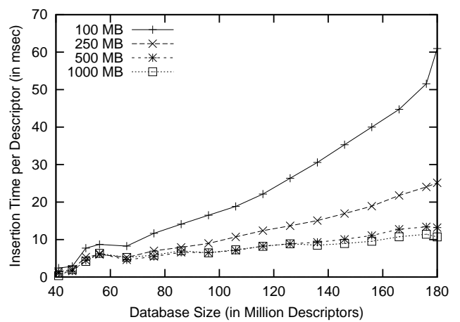
Fig. 9. Average time to insert a descriptor as the index grows, for various buffer sizes.
